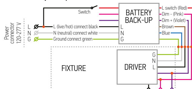
UHB5-HV with battery back-up kit
