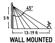
WALL MOUNTED
